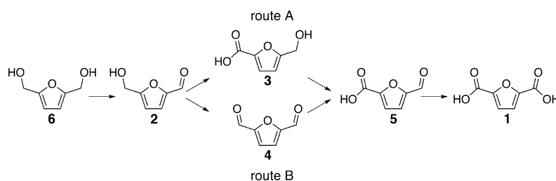
Scheme 1. The oxidation of [5-(hydroxymethyl)furan-2-yl]methanol ( 6 ) and 2 into the diacid 1 can proceed by two routes. Route A: the aldehyde group of 2 is oxidized to form a carboxylic acid. Route B: the alcohol group of 2 is oxidized to yield the dialdehyde 4 . HMFO exclusively uses route B. Each step is a two-electron oxidation in which one equivalent of O 2 is consumed and one equivalent of H 2 O 2 is formed by the enzyme.
