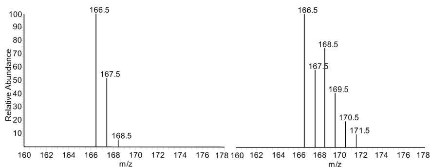
Figure 1. APCI-MS (negative mode) of HMFO-formed 4-nitrobenzoic acid. The spectrum on the left shows the product formed in \text{H}_2\text{O} , and the spectrum on the right shows the increased masses of 168 and 170 ( M+2 and +4 respectively) when oxidation of 4-nitrobenzaldehyde was performed in 30% \text{H}_2^{18}\text{O} .
